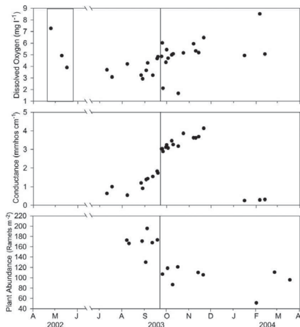
Fig. 2. Dissolved oxygen, specific conductance, and plant abundance monitoring over time at the Dow Wetland 2003 mechanical shredding station (D1). The black rectangle before the scale break indicates a time period when water hyacinth invaded the station area (April–May 2002). The black vertical line indicates when mechanical shredding was conducted on the station with the AquaPlant Terminator.
