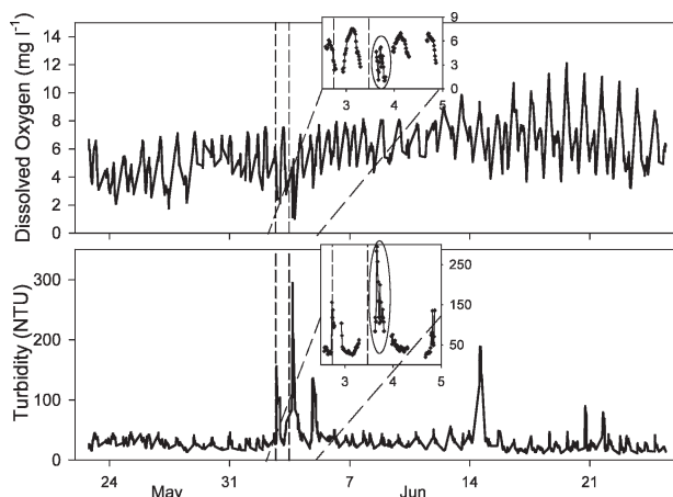
Fig. 4. Continuous monitoring of dissolved oxygen and turbidity in the Dow Wetland mechanical shredding station (D1) during a one month period in 2004. The vertical hash lines indicate points when mechanical shredding was conducted on the site using the Cookie Cutter. Inset plots present on an expanded time scale the 48-h period when the shredding operation was conducted, with the circled area referred to in the text.
