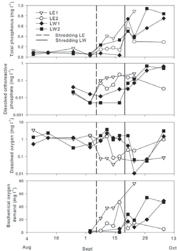
Fig. 3. Results of the water chemistry monitoring over time for Lambert Slough monitoring stations in 2003. The dashed vertical line indicates the date of Amphibious Terminator shredding in East Lambert Slough. The two East Lambert Slough stations are LE1 ( \nabla ) and LE2 ( \circ ). The solid vertical line indicates the date of AquaPlant Terminator shredding in West Lambert Slough. The two West Lambert Slough stations are LW1 ( \blacklozenge ) and LW2 ( \blacksquare ). Note log axes, second and third plots.
