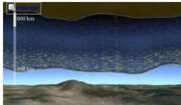
The height of the ionosphere/space transition is controlled in part by the amount of extreme ultraviolet energy emitted by the Sun and a somewhat contracted ionosphere could have been expected because C/NOFS was launched during a minimum in the 11-year cycle of solar activity. However, the size of the actual contraction caught investigators by surprise. (Credit: NASA/Goddard Space Flight Center)
