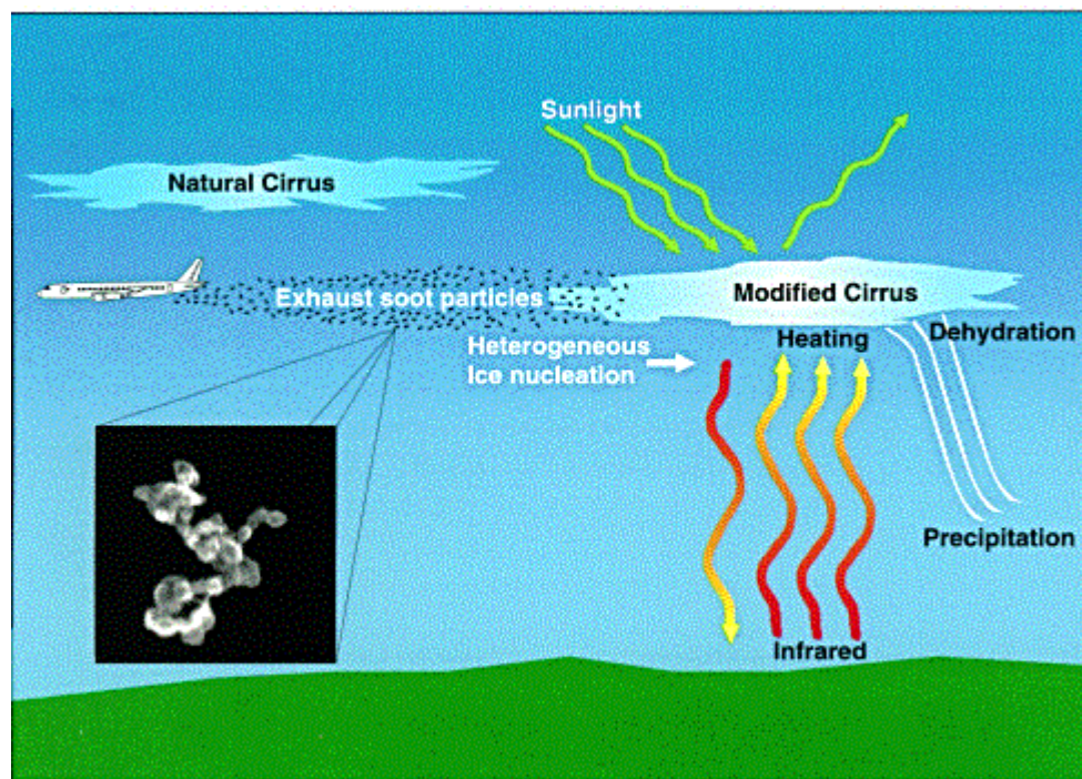
Figure 1: Ice cloud microphysical model
