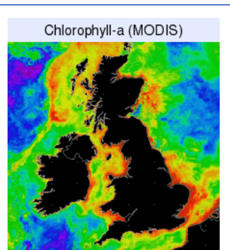
Example NEODAAS products and data illustrating the range of sensors that we are able to both receive and process data from.
