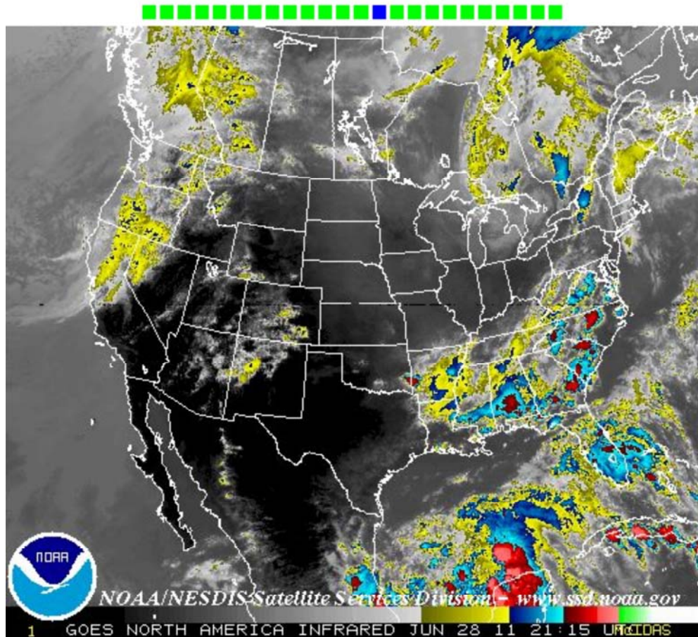
1 GOES NORTH AMERICA INFRARED JUN 28 11 21:15 UTC/CDAS
