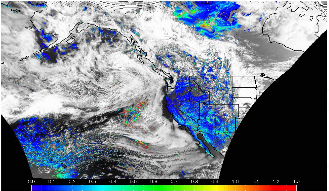
GASP West Aerosol Optical Depth 01:15UTC 6/21/2011
