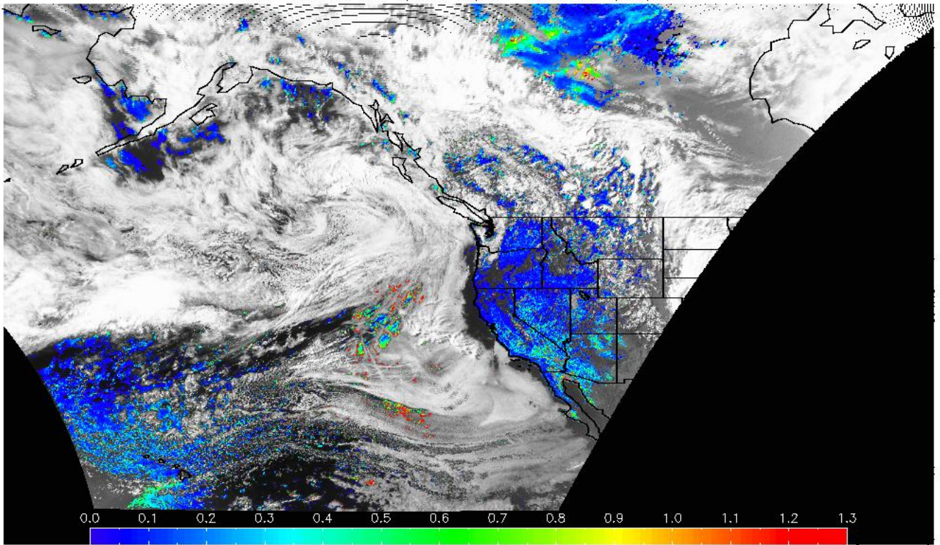
GASP West Aerosol Optical Depth 01:45UTC 6/21/2011
