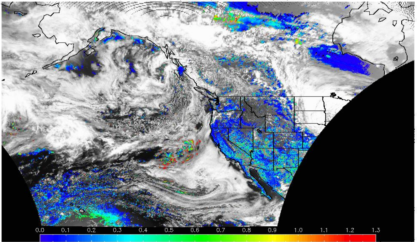
GASP West Aerosol Optical Depth 23:45UTC 6/21/2011
