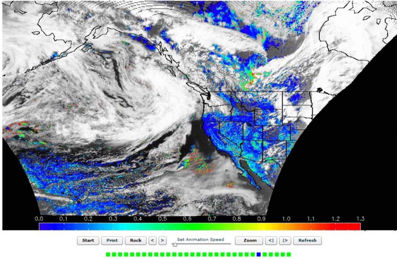
GASP West Aerosol Optical Depth 01:15UTC 6/27/2011
