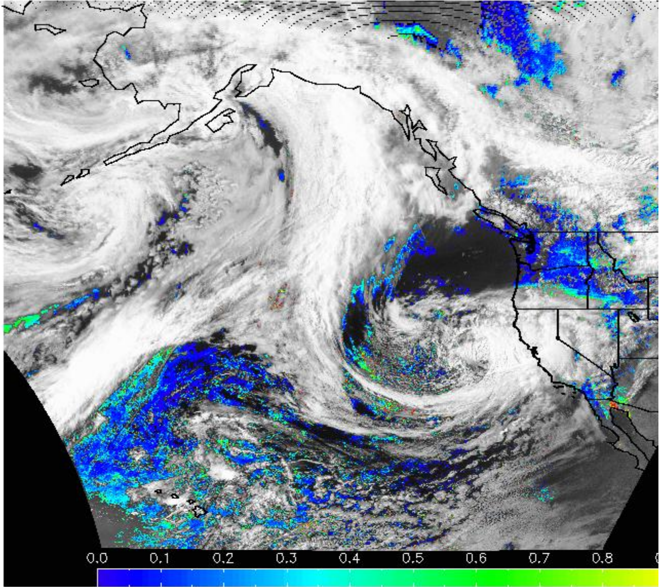
GASP West Aerosol Optical Depth 01:45UTC
