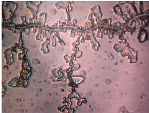
Crystalline formations in saliva, 700x magnification
